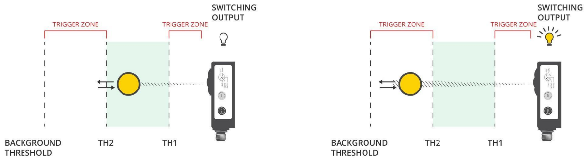
Figure 15. Mode 3 operation for NO/NC Active region = 1 ⇒ Only white patched areas (Th2 < distance OR distance < Th1) are triggering the switching output
