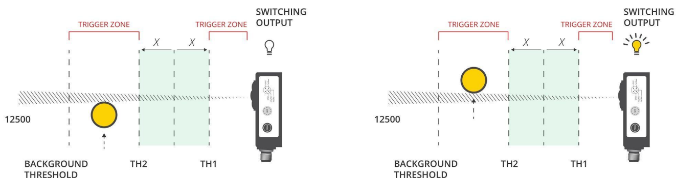
Figure 21. Mode 5 operation (NO/NC active region = 1) ⇒ Only white patched areas ( Th2 < \text{distance} OR \text{distance} < Th1 ) are triggering the switching output
