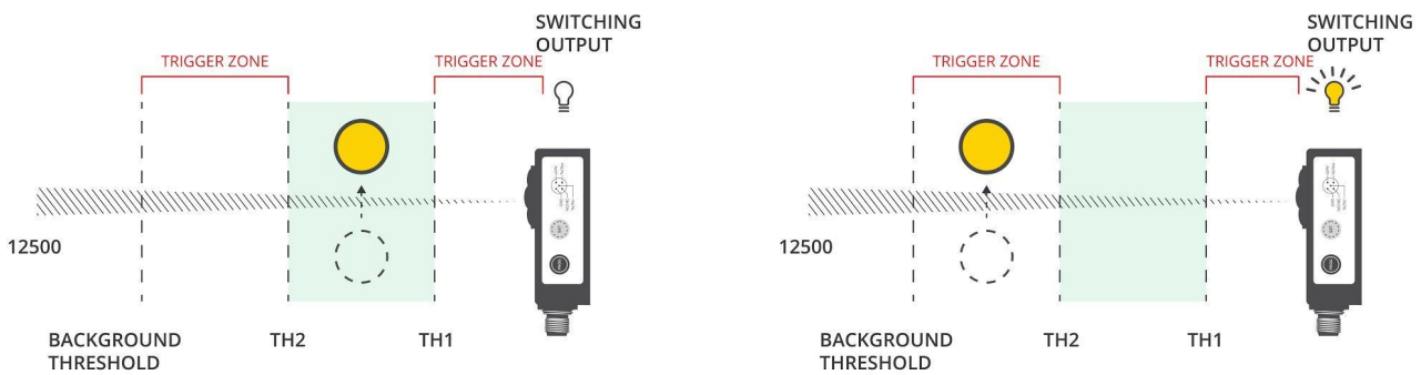
Figure 18. Mode 4 operation (NO/NC active region = 1) ⇒ Only white patched areas (Th2 < distance OR distance < Th1) are triggering the switching output
