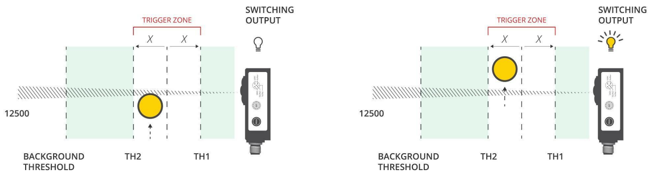
Figure 20. Mode 5 operation (NO/NC active region = 0) ⇒ Only white patched area ( Th1 < \text{distance} < Th2 ) is triggering the switching output
