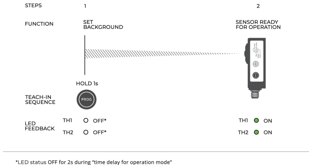
Figure 9. Mode 1 setup phases
