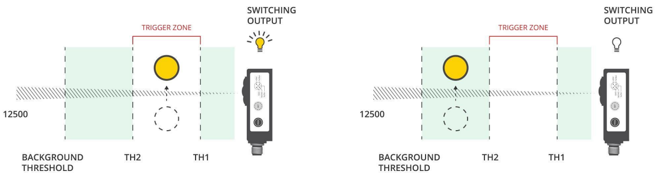
Figure 17. Mode 4 operation (NO/NC active region = 0) ⇒ Only white patched area (Th1 < distance < Th2) is triggering the switching output
